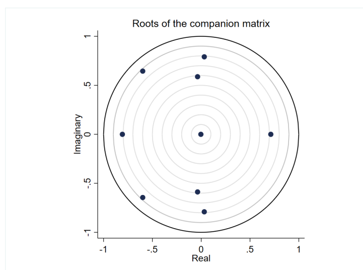
Figure 10: Unit circle inspection chart
