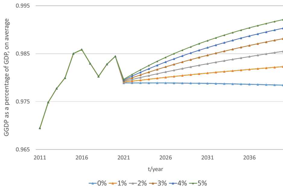
Figure 12: Stability test of \theta
